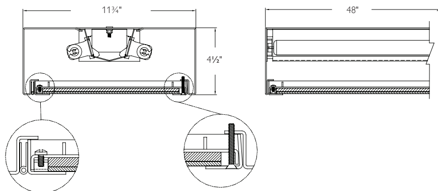
Piano hinge design on medium security models.
